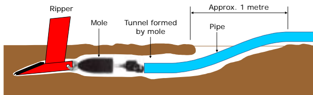
Laying poly pipe with the mole drainer
